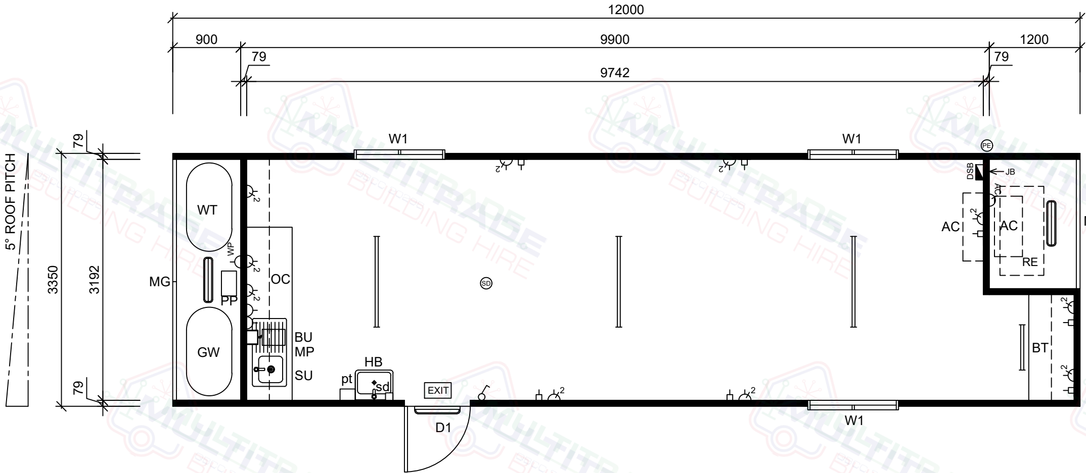
12.0x3.35m Site Office (*SOLAR) - Floor Plan Scale 1:50
